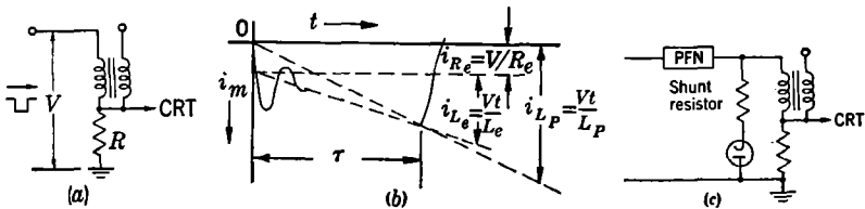
FIG. 12-8.—Method of measurement of primary inductance.
